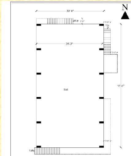
PLAN SHOWING PROPOSED CELLAR FLOOR PLAN CONSTRUCTION OF GURUKULA BUILDING AT SRIRANGAPATTANA.
