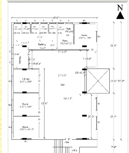
PLAN SHOWING PROPOSED FIRST FLOOR PLAN CONSTRUCTION OF GURUKULA BUILDING AT SRIRANGAPATTANA.
