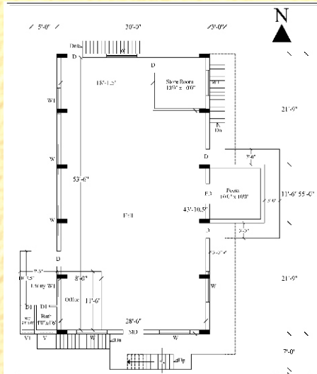
PLAN SHOWING PROPOSED GROUND FLOOR PLAN CONSTRUCTION OF GURUKULA BUILDING AT SRIRANGAPATTANA.
